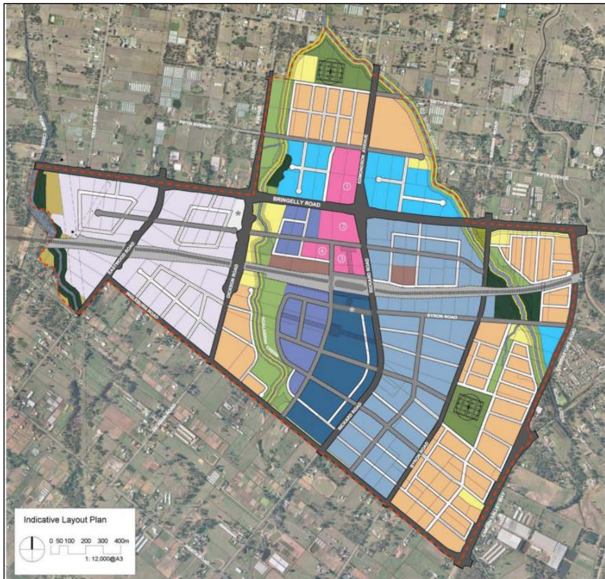
Image 1 – Indicative Layout Plan
